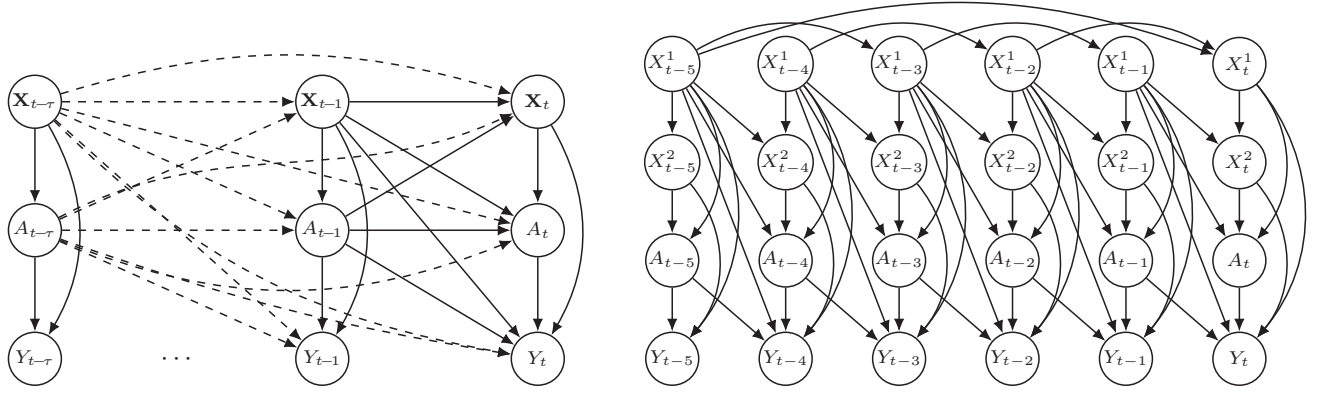
(a) Window causal graph structuring the fully synthetic DGP over a temporal window of size \tau \in \{1, 3, 5, 30\} . The lag- \tau arrows from A_{t-\tau} to X_t and A_t follow the DGP equations in Appendix D.2.
