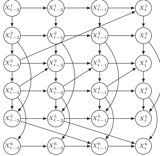
Figure 6: Window causal graph structuring the fully synthetic DGP ( \tau=3 ) used in ablation study experiments.
