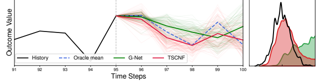
Figure 4: Simulated 5-step-ahead history-adjusted interventional trajectories and the final step density plot in the sparse temporal dependency setting.
