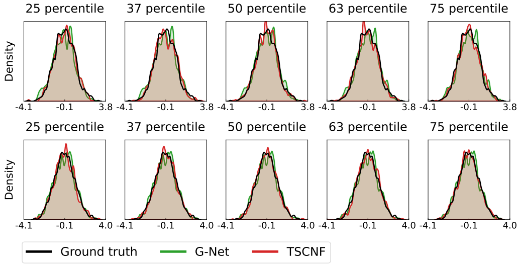
Figure 11: Density plots of the history-adjusted interventional distributions P(Y_{m+3}(a_{m+1}) | \bar{x}_m) under various time-varying treatment strategies in the linear (top) and the non-linear (bottom) dataset ( \tau = 30 ).
